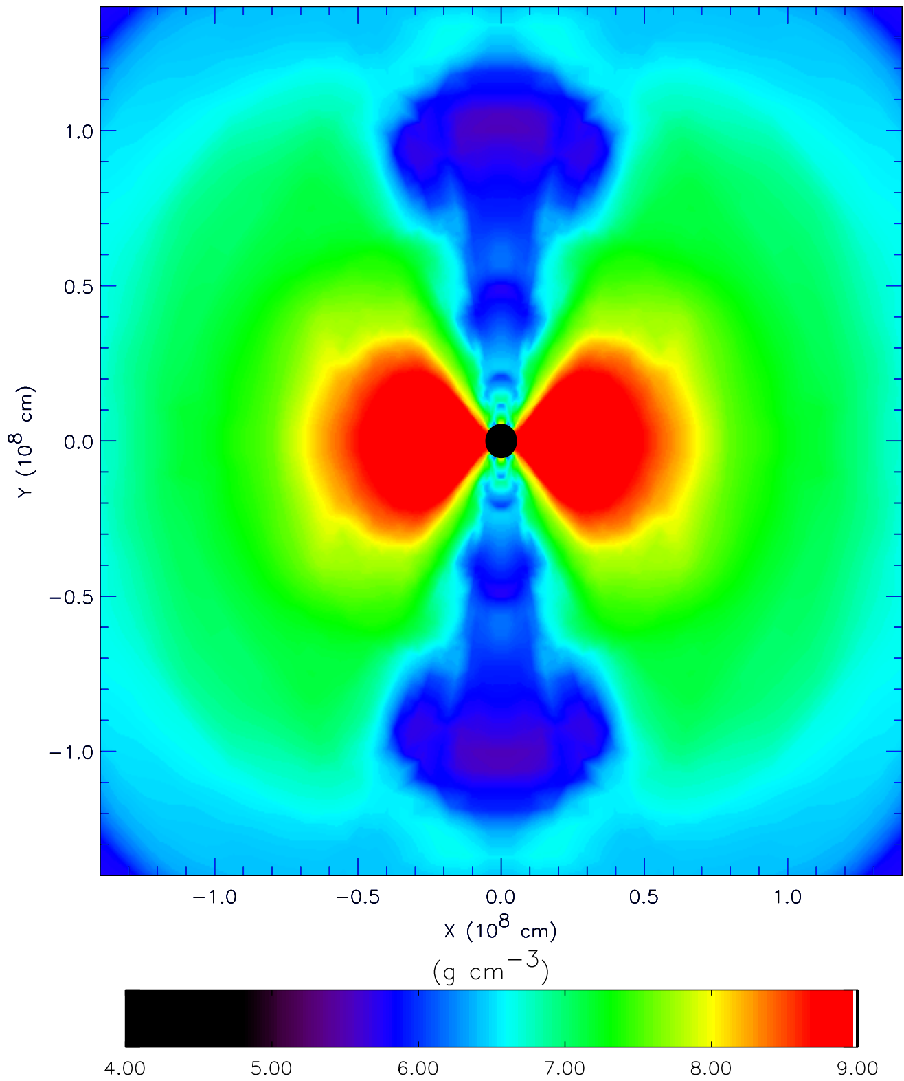
MacFadyen, Woosley, & Heger (1999)
