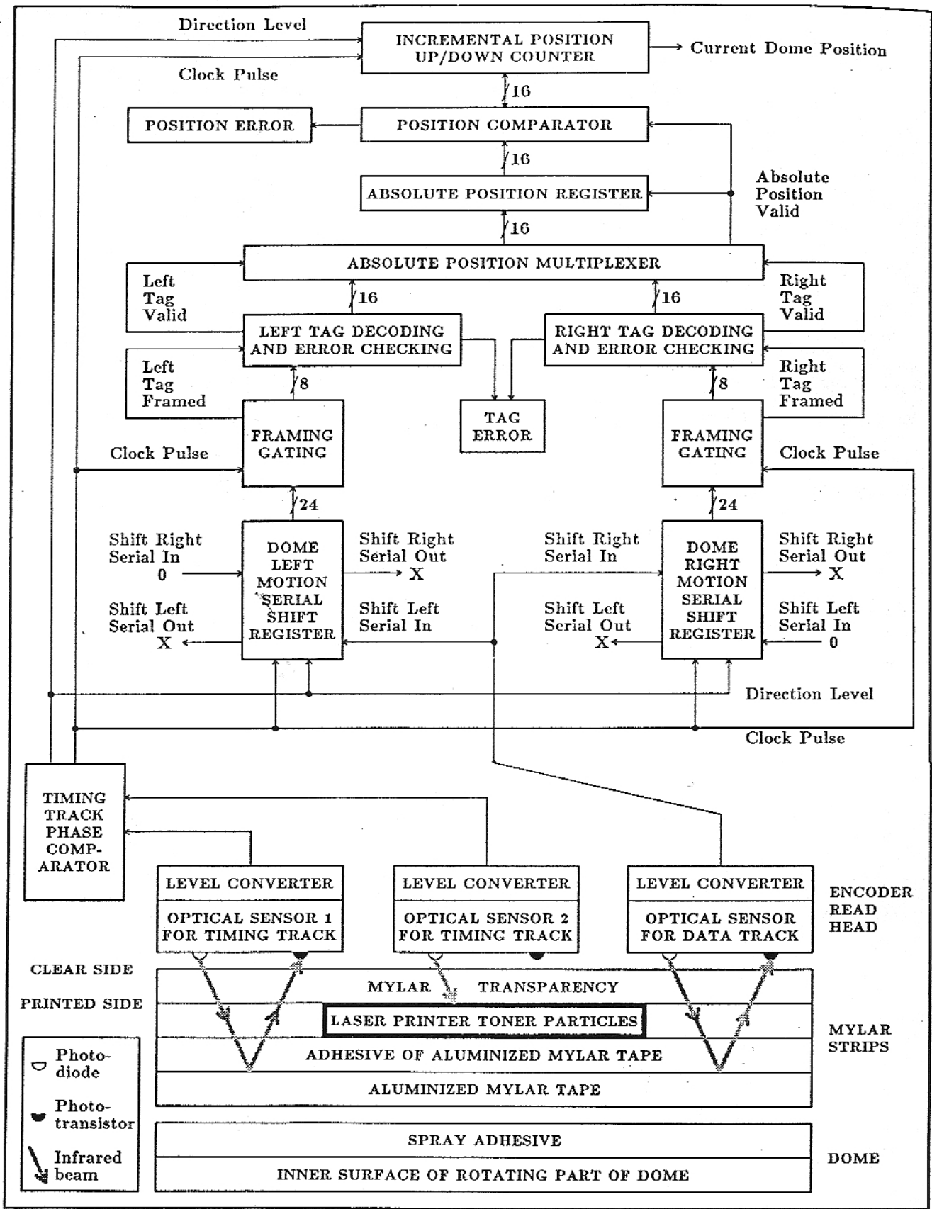
Figure 2. Block diagram of hybrid encoder system.
