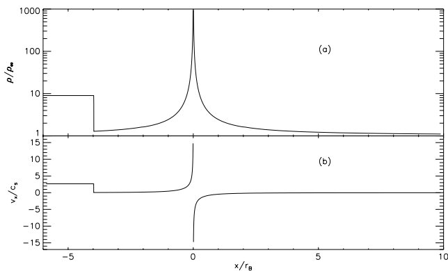
FIG. 12.—(a, b) Density and x -velocity, respectively, along the x -axis in the initial configuration of our Bondi to Bondi-Hoyle accretion problem. The Bondi radius, sound speed, and background density are r_B = 0.12 pc, c_s = 0.19 km s ^{-1} , and \rho_\infty = 10^{-25} g cm ^{-3} .
