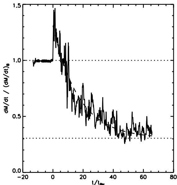
FIG. 14.—Solid curve: Accretion rate onto the sink particle vs. time, sampled at intervals of t_{\text{BH}}/10 . Short-dashed horizontal lines: Predicted Bondi (upper line) and Bondi-Hoyle (lower line) accretion rates. Long-dashed line: Exponential fit to the accretion rate after the shock hits the sink particle. Time is plotted in units of t_{\text{BH}} = 6.35 \times 10^4 yr, and accretion rate is plotted in units of \dot{M}_B = 5.9 \times 10^{-11} M_\odot \text{ yr}^{-1} .
