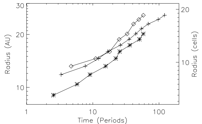
FIG. 8.—Radius of the evacuated region vs. time in simulations of disk evolution around a sink particle. Line marked with diamonds : Run without sink particle accretion. Line marked with crosses : Run with accretion that is stationary relative to the grid. Line marked with asterisks : Run with the sink particle advected relative to the grid.
