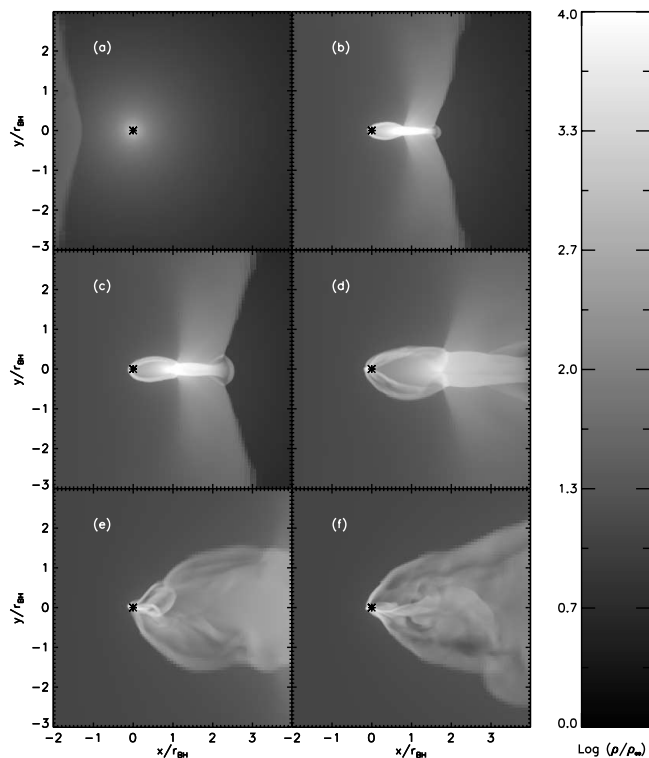
FIG. 13.—Series of slices through the equatorial plane. The density range has been truncated to bring out detail. The asterisks indicate the position of the sink particle; we do not show the accretion region because it is too small to see clearly. We have truncated the density range at the top and the bottom to bring out details. Note that in contrast with Figs. 11 and 12, the length unit of these plots is r_{\text{BH}} = 0.012 pc = r_B/10 . The times shown in each panel are as follows: (a) -0.25t_{\text{BH}} , (b) 1.6t_{\text{BH}} , (c) 1.9t_{\text{BH}} , (d) 2.7t_{\text{BH}} , (e) 4.3t_{\text{BH}} , and (f) 5.9t_{\text{BH}} , where t_{\text{BH}} = 6.35 \times 10^4 yr. [See the electronic edition of the Journal for a color version of this figure.]
