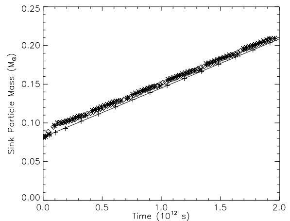
FIG. 2.—Mass of the sink particle vs. time. Solid line : Theoretical result. Crosses : Values from the unadvected run. Asterisks : Values from the run advected at Mach 0.5. Diamonds : Values from the run advected at Mach 2.
