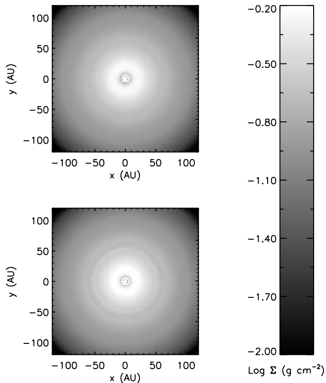
FIG. 5.—Surface density of our simulated disks after a time of \approx 50 orbital periods at the edge of the accretion zone, r = 5.55 AU. Top : Run with the sink particle stationary on the grid. Bottom : Run with the sink particle advected across the grid. The white outlines in the center of each plot show the accretion zone. In the bottom panel, x - and y -coordinates are measured relative to the sink particle's position. [See the electronic edition of the Journal for a color version of this figure.]
