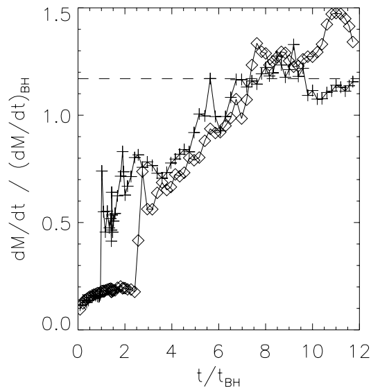
FIG. 4.—Accretion rate as a function of time in our simulations of Bondi-Hoyle accretion. The points are sampled at intervals of \sim t_{\text{BH}}/5 . Time is plotted in units of t_{\text{BH}} = 6.35 \times 10^4 yr, and accretion rate is plotted in units of \dot{M}_{\text{BH}} = 1.7 \times 10^{-12} M_{\odot} \text{ yr}^{-1} . Crosses : Simulation with the sink particle stationary. Diamonds : Simulation with the sink particle moving. Dashed horizontal line : Accretion rate predicted by Ruffert (1996).
