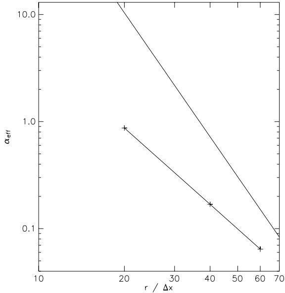
FIG. 10.—Plot showing \alpha approximated using our disk evacuation method (upper, unmarked line) and using our ring method (lower line, marked with crosses).
