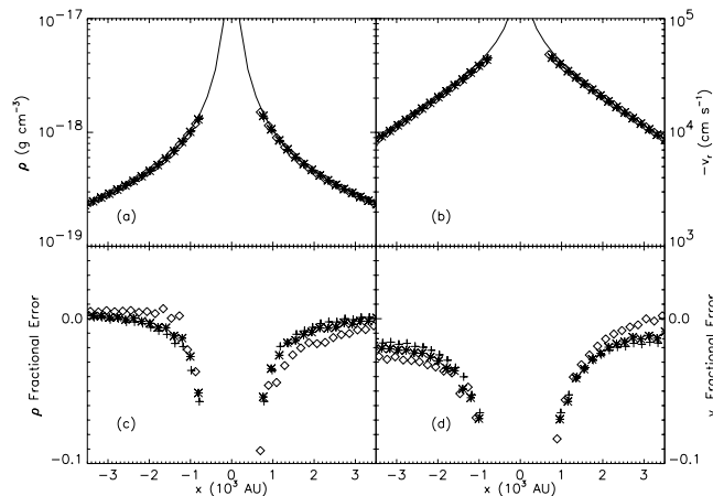
FIG. 1.—Results of our isothermal sphere test. (a, b) Density and velocity vs. radial distance in the sink particle’s rest frame. (c, d) Fractional error in density and velocity. All quantities are plotted along the direction of the sink particle’s motion. In the top panels, the analytic solution is the solid line. In all panels the crosses show values from the unadvected run, the asterisks show values from the run advected at Mach 0.5, and the diamonds show values from the run advected at Mach 2. The simulation data stop at the edge of the sink region. All the plots are at time t = 2.0 \times 10^{12} s.
