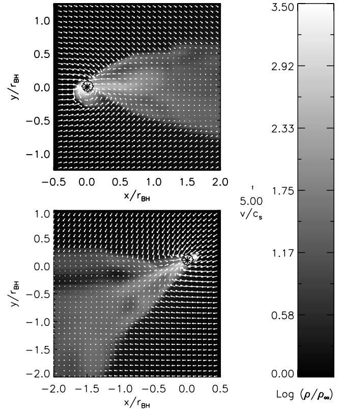
FIG. 3.—Density and velocity fields in the xy -plane at t \approx 12t_{\text{BH}} . Top : Run with the sink particle at rest. Bottom : Run with the sink particle moving relative to the grid. The bottom plot is in a coordinate system comoving with the sink particle. The black borders indicate the boundary of the accretion zone. [See the electronic edition of the Journal for a color version of this figure.]
