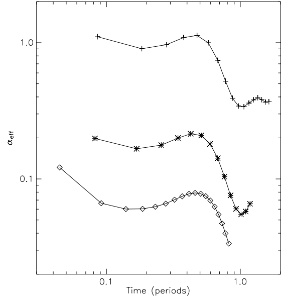
FIG. 9.—Best-fit value of \alpha vs. time for our ring test. The curves marked with crosses, asterisks, and diamonds are for r/\Delta x = 20, 40, and 60, respectively. The x -axis measures time in units of orbital periods at the initial radius of the ring.
