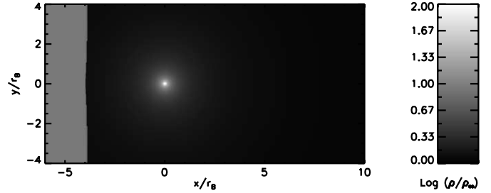
FIG. 11.—Logarithm of density for the initial configuration of the Bondi-Hoyle accretion problem. The image is a slice through the equatorial plane. We do not show the accretion region or sink particle because they are too small to see clearly. The plotted density range has been truncated at the top to bring out lower density features. The small irregularity visible in the shock front is a result of varying resolution: the shock is wider farther from the x -axis because it is spread over \sim 3 cells and the cells are larger farther from the axis. The Bondi radius is r_B = 0.12 pc; \rho_\infty = 10^{-25} g cm ^{-3} . [See the electronic edition of the Journal for a color version of this figure.]
