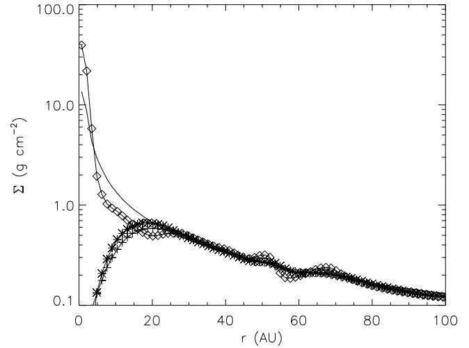
FIG. 7.—Azimuthally averaged surface density vs. radius after 50 orbital periods at the edge of the accretion region, r = 5.55 AU, in simulations of disk evolution around a sink particle. Line marked with diamonds : Run without sink particle accretion. Line marked with crosses : Run with accretion where the sink particle is stationary with respect to the grid. Line marked with asterisks : Run with the sink particle advected relative to the grid. Unmarked line : Initial surface density profile. The interval in radius between data points is one cell.
