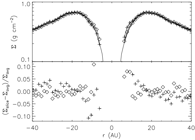
FIG. 6.— Top : Azimuthally averaged surface density (unmarked line), surface density sliced along the sink particle’s direction of motion (line with crosses), and surface density sliced transverse to the direction of motion (line with diamonds) for our run with the sink particle advected across the grid. Bottom : Fractional difference between the slice and the azimuthal average. The data for the slices end at the edge of the accretion zone. The distances r are measured relative to the position of the sink particle. The plots are for a time of \approx 50 orbital periods at the edge of the accretion zone, r = 5.55 AU.
