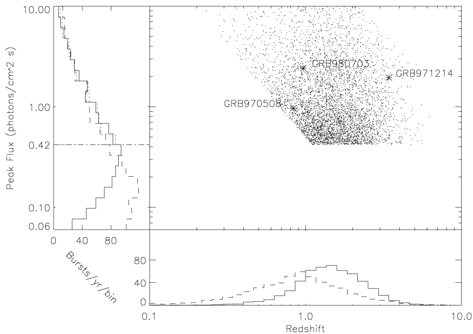
FIG. 2.—The largest panel shows the points indicating the peak flux and redshift for 5000 GRBs selected from the SFR distribution with the BATSE flux cutoff; the asterisks are GRB 970508, GRB 971214, and GRB 980703. The left panel shows the number of GRBs per year in each peak flux range, divided into 20 evenly spaced logarithmic bins. The dot-dashed horizontal line shows the BATSE flux cutoff. The histogram in the bottom panel shows the expected number of bursts per year in each redshift range, divided into 30 evenly spaced logarithmic bins. The total number of bursts is generated by setting the number in each model equal to the number per year seen by BATSE, corrected for BATSE's effective coverage of 48.3% of the sky. In the left and bottom panels, the solid histogram is the SFR model, and the dashed histogram is the CCD model. The dotted line in the left panel is the BATSE catalog.
