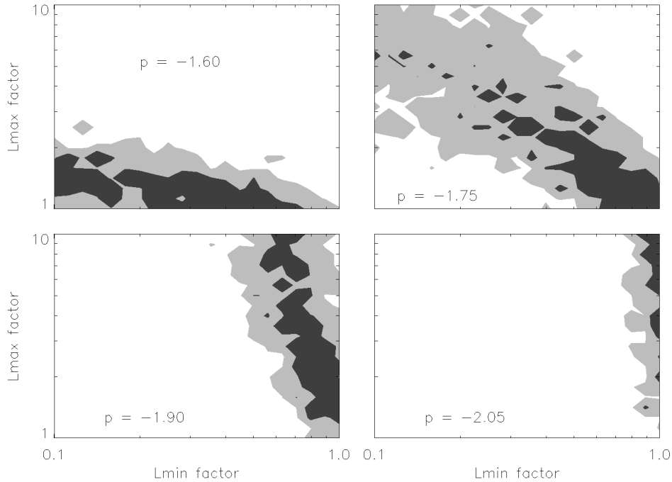
FIG. 1.—The light contour shows models with significance greater than 0.05, and the dark contour shows models with significance greater than 0.33. One minus the significance value is the confidence level at which the model can be ruled out. The L_{\min} factor and the L_{\max} factor indicate the amount by which the luminosities of GRB 970508 and GRB 971214 are multiplied, respectively. Values of p , the exponent of the luminosity distribution, are indicated in each panel.
