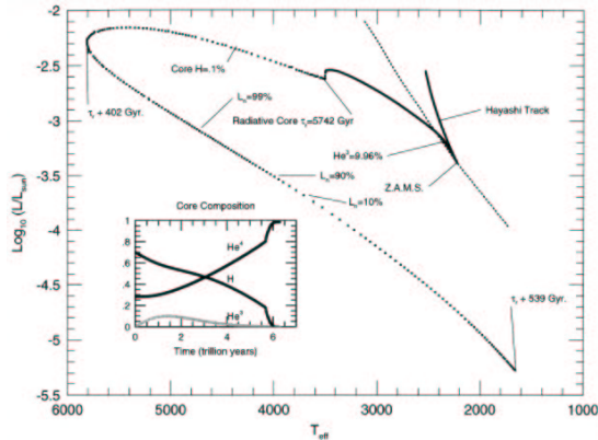
Fig. 1. Evolution in the H-R diagram for a small M Dwarf star with mass M_* = 0.1M_\odot (from LBA). Each small circle in the track represents a converged stellar model. This track starts with the pre-main-sequence Hayashi track and ends with a white dwarf cooling track several trillion years later. The inset diagram shows the chemical composition of the star as a function of time.
