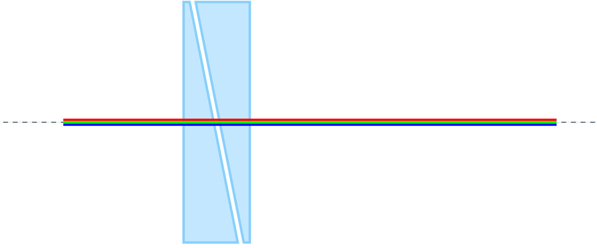
Linear ADC, conceptual. Prism separation controls image offset.
