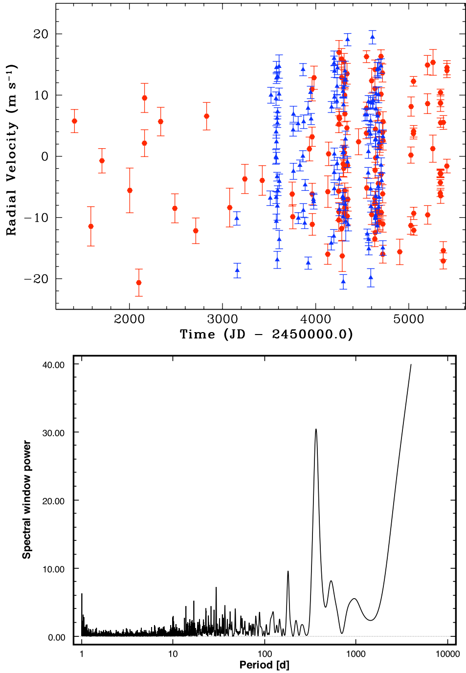
Fig. 2.— Top panel: Combined RV data of GJ 581 from HIRES (red hexagons) and HARPS (blue triangles). Lower panel: spectral window
