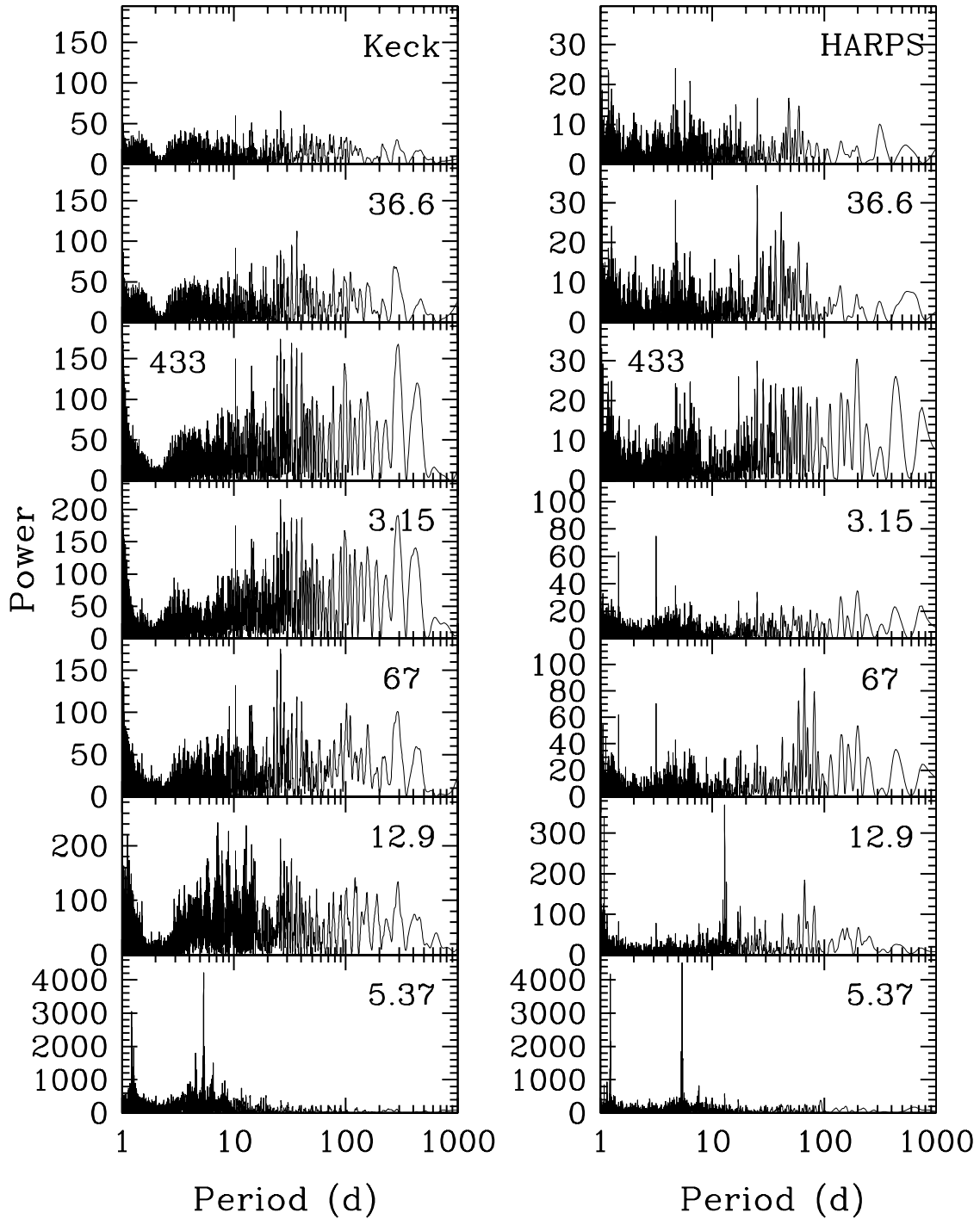
Fig. 4.— The effect of adding signal at each Keplerian period back into the residuals of each data set for GJ 581. The panels on the left show results for the HIRES data set, while those on the right show results for the HARPS data set. The top panel on each side shows the periodogram of the residuals from the 6-planet fit. Descending panels shows the effect of injecting the known signal from each Keplerian period back into the residuals.
