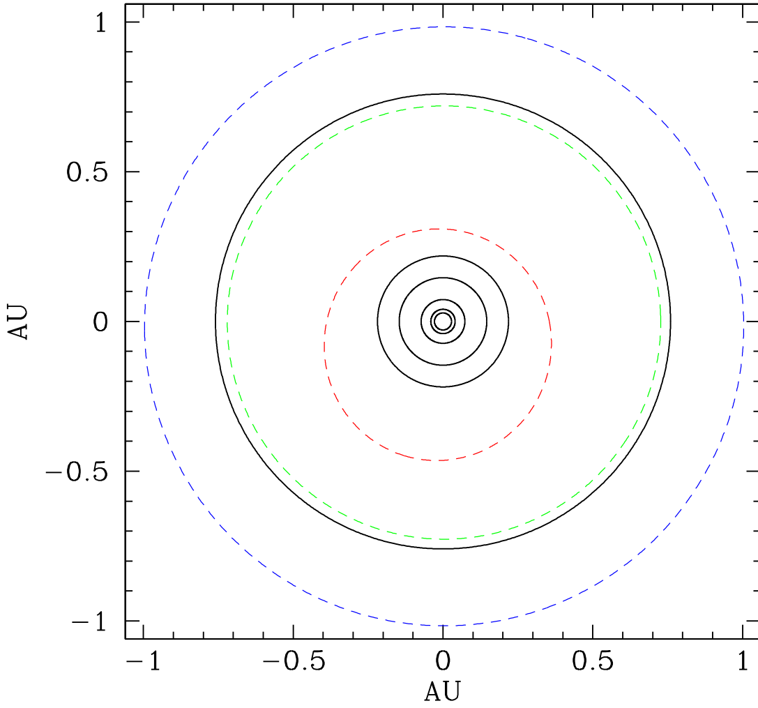
Fig. 6.— Top view of the GJ 581 system. For reference, the orbits of Earth, Venus, and Mercury are overlaid as dashed blue, green, and red lines respectively.
