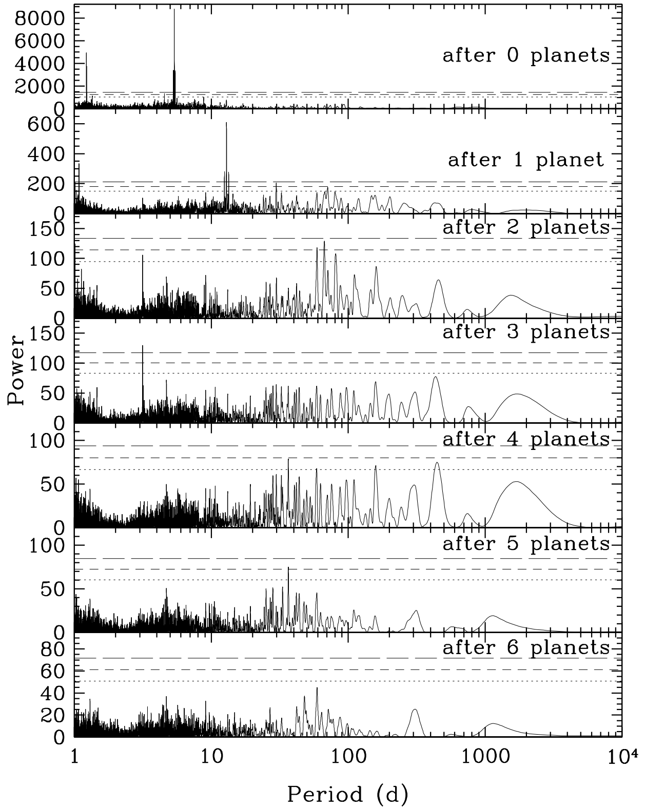
Fig. 3.— From top to bottom, power spectra of the residuals to the 0-, 1-, 2-, 3-, 4-, 5-, and 6-planet solutions, respectively.
