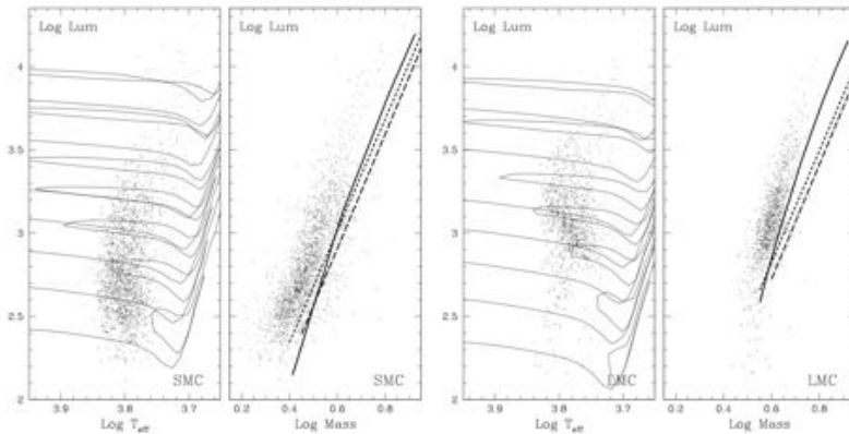
Fig. 5. Theoretical HR diagram and Mass-luminosity relations for SMC (the two left panels) and for LMC (the two right panels). As in Fig. 4, fundamental Cepheids are shown as solid circles and overtones as open circles. Calculations: Theoretical HR diagram with superposed evolutionary tracks from Girardi et al. (2000). M-L relations from evolutionary calculations; solid lines: Girardi et al. 2000, dotted lines: Alibert et al. 1999, dashed lines: Bono et al. 2000.
