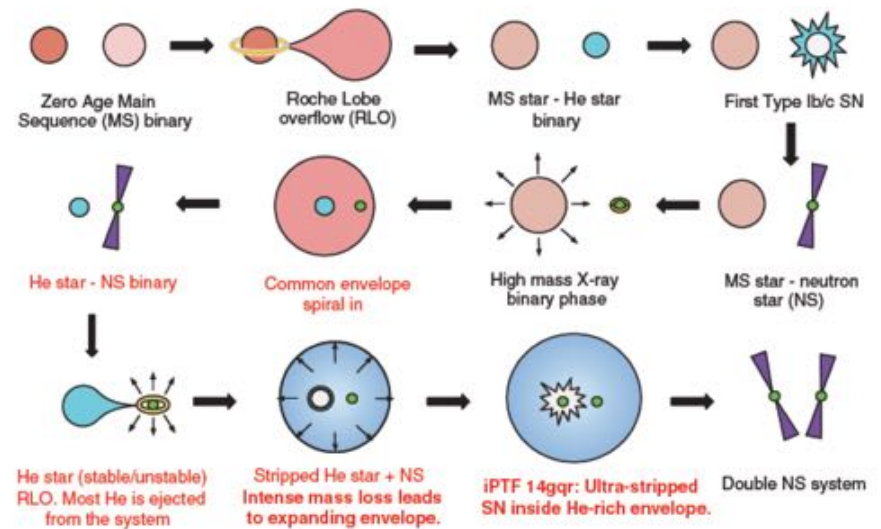
Complex stellar evolution
