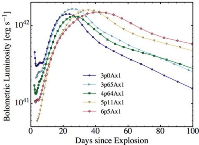
(Common) Type Ib and Ic supernovae
