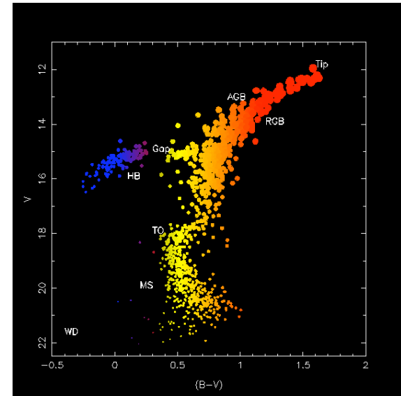
TO = “turn off mass”; HB = “horizontal branch”; “Gap” is a region of atmospheric instability
