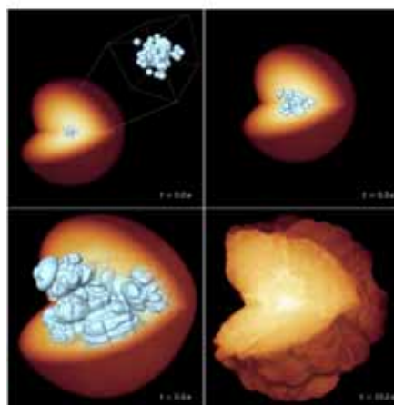
Roepke and Hillebrandt (2007)
