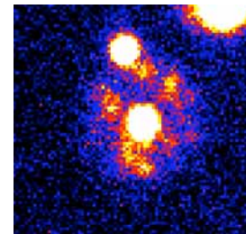
Nova Cygni (1975) V1500 Cygni
