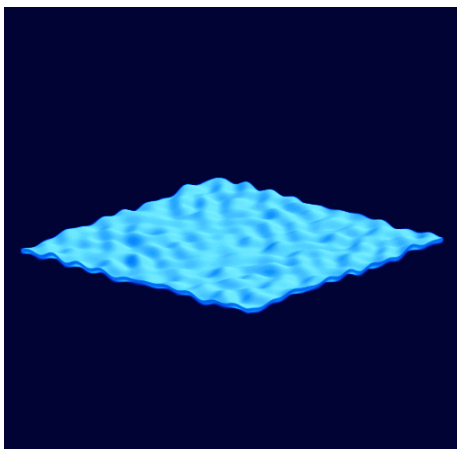
Zingale et al. (2005)
