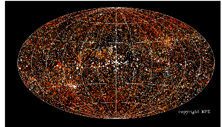
ROSAT – first pass in 1990 – 1991 50,000 sources. By 1999 over 150,000 sources had been catalogued.
