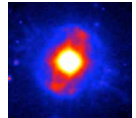
Nova Pictoris (1927) RR Pic
