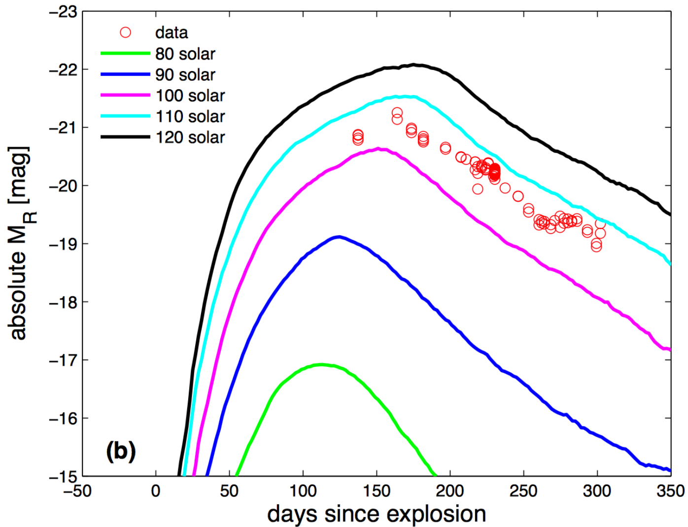
SN 2008bi - GalYam et al, Nature, (2009) reported as a pair-instability supernova. Data compared with models by Kasen, Woosley and Heger (2002, 2008)
