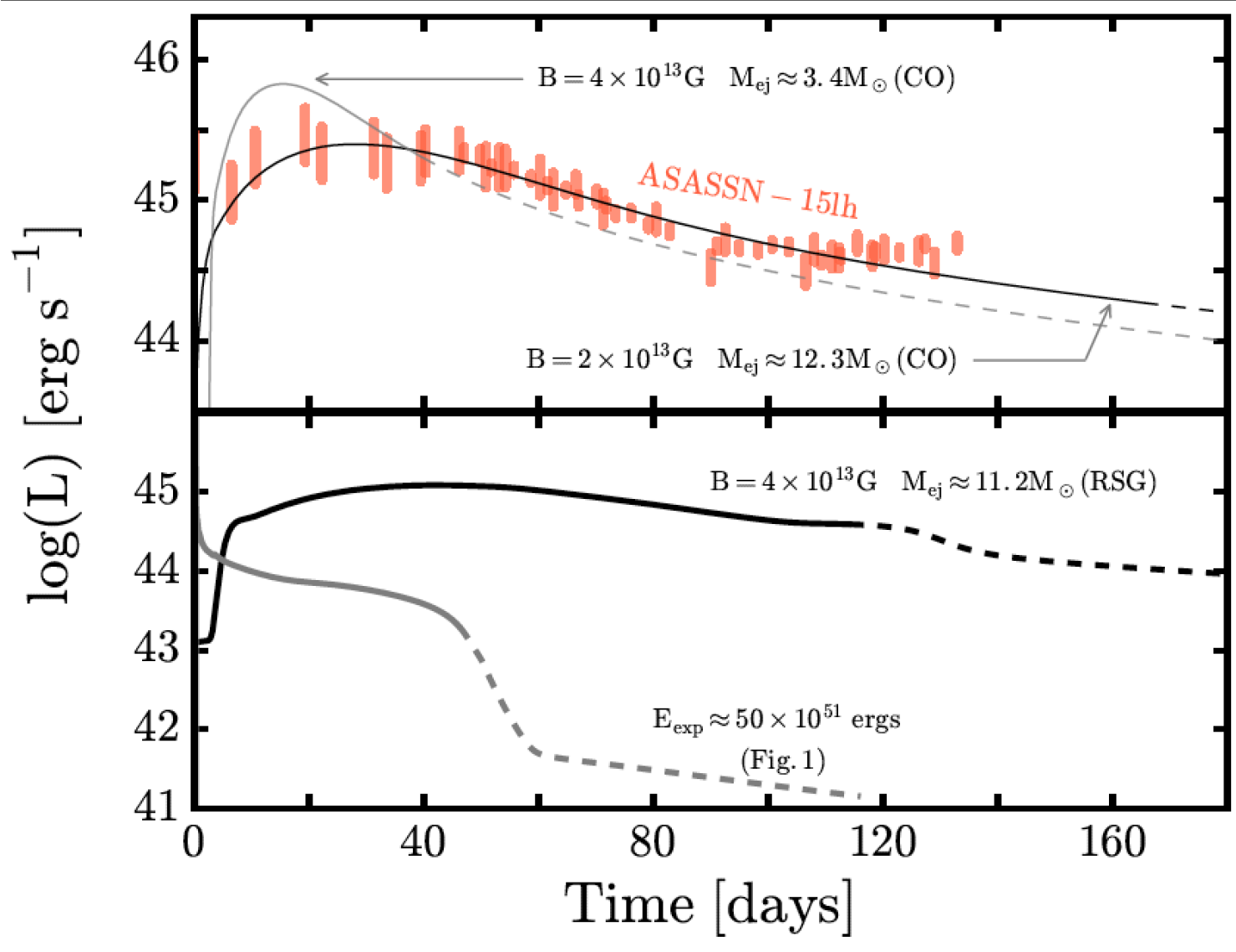
Brightest SN ever!! Model by Sukhbold and Woosley (2016)
