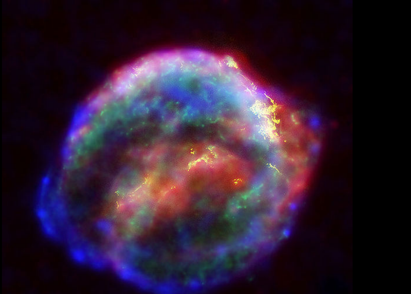
Kepler's supernova remnant in the optical (HST yellow), IR (Spitzer (red)), and x-ray (Chandra, blue and green). Blue and yellow are shocked gas, green is hot gas, red is dust.
