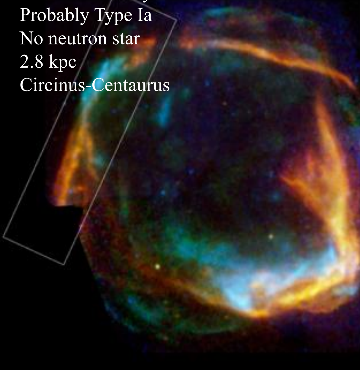
XMM FULL-FIELD
