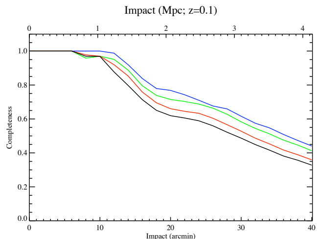
FIG. 5.— Completeness curves for the galaxy survey as a function of impact parameter to the quasar. The curves refer to limiting magnitudes R_{lim} = 18, 19, 19.5, 20 \text{ mag} . The measurement is a direct evaluation for galaxies within 10' of the quasar. At radii greater than 10' , the incompleteness is primarily due to the discontinuous coverage of the flanking fields (Figure 2). At these radii, we used the surface density of objects within 10' to estimate the incompleteness in the discontinuous regions.
