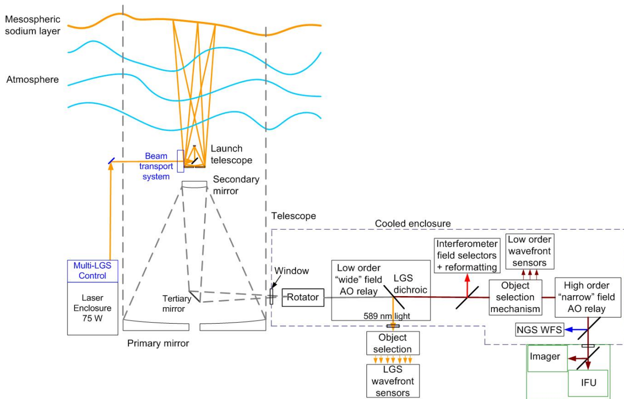
Figure 9. Schematic of the NGAO concept
