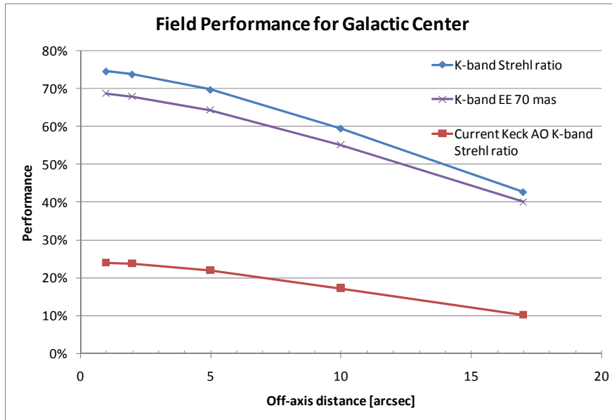
Figure 13. NGAO Strehl ratio and ensquared energy (in a 70x70 mas area) for the Galactic Center science. The maximum off-axis distance is 2" for integral field spectroscopy and 5" for imaging of the Galactic Center.
