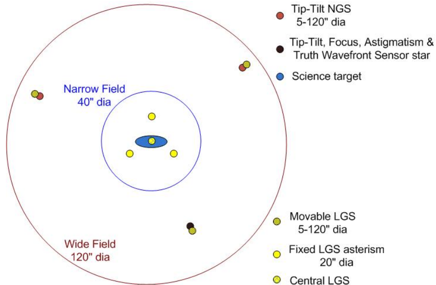
Figure 10. Schematic of the NGAO LGS asterism
