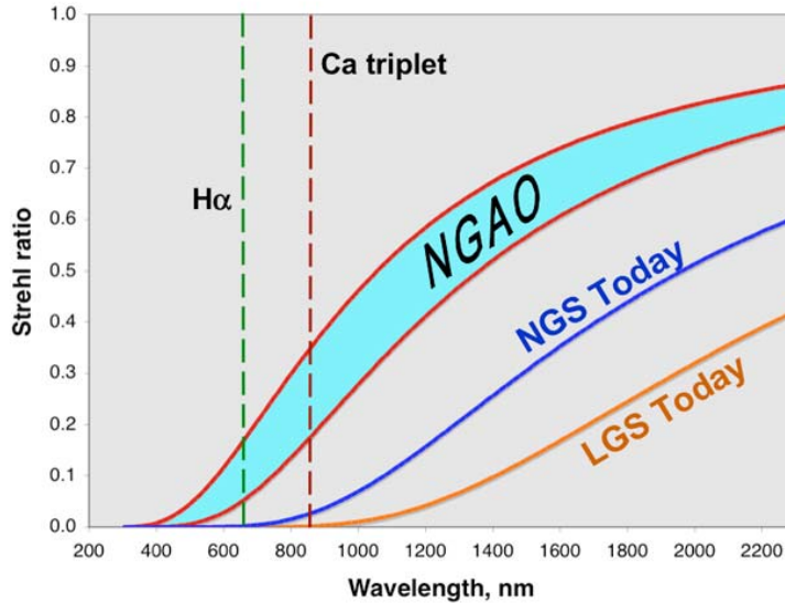
Figure 14. NGAO versus current Keck II NGS and LGS AO performance (for the case when a bright natural guide star is available for NGS AO or for tip-tilt correction with LGS AO).
