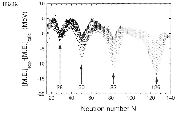
Fig. 1.11 Difference between experimental ground-state atomic mass excess (Audi et al. 2003) and the mass excess predicted by the spherical macroscopic part of the finite-range droplet (FRDM) mass formula (Möller et al. 1995) versus neutron number.
