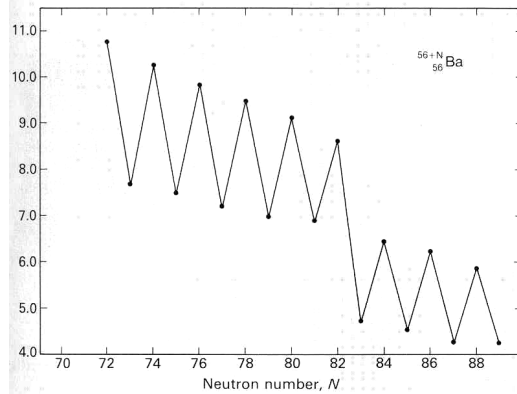
Ba Neutron separation energy in MeV
