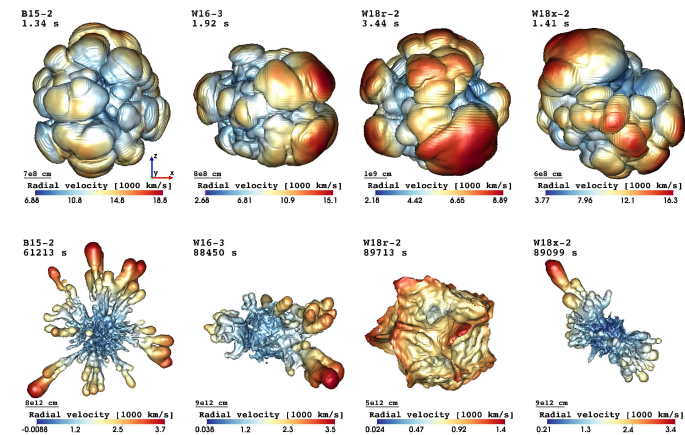
^{56}\text{Ni} -rich material at two times in 4 3D models
