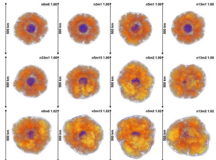
Figure 1. Volume renderings of specific entropy for several of the 3D simulations at 150ms after bounce. Darker, red colors correspond to specific entropies of \sim 14 k_B baryon -1 while lighter, yellow colors correspond to entropies of \sim 18 k_B baryon -1 . The blue colors, which highlight the shock surface and the lower-entropy cooling region near the proto-neutron star, correspond to specific entropies of \sim 5 k_B baryon -1 . Models with stronger perturbations show higher specific entropies in the gain layer and a greater shock extension. This is a result of the stronger turbulence and concomitant higher neutrino heating efficiency and turbulent pressure in these models.
