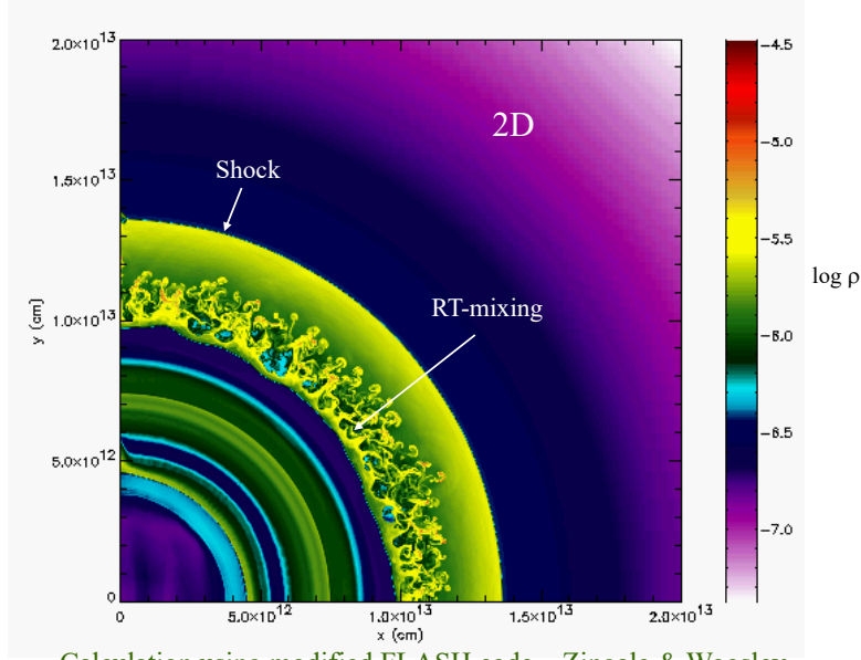
Calculation using modified FLASH code – Zingale & Woosley
