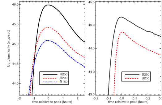
Figure 3. Calculated bolometric light curves of the shock breakout transient from pair instability explosions of massive red-supergiant (left) and blue-supergiant (right) stars. The duration of the burst, determined by the light crossing time, is significantly longer for the more extended red-supergiant models. (A color version of this figure is available in the online journal.)
