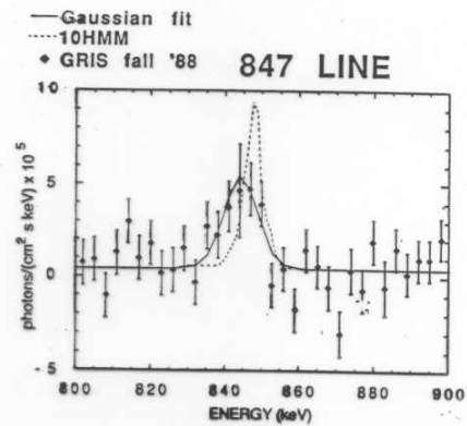
Figure 2. GRIS data for the 847 keV line from the decay of ^{56}\text{Co} in SN1987A is shown for day 613. The top-of-atmosphere photon spectrum is shown in 3 keV bins which are larger than the FWHM resolution of the instrument. The solid line is a best fit to a Gaussian line profile. The dashed line is the predicted line profile for the 10HMM model. Although this model and similar spherically symmetric mixed models predict the line flux correctly there is a clear discrepancy with the measured line profile.
