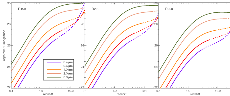
Figure 17. Detectability of the shock breakout transient from pair instability supernovae as a function of redshift. The figure plots the observed AB magnitude (for different wavelength bands) of three red-supergiant models at the peak of the bolometric breakout light curve. (Note an AB magnitude of 28.9 corresponds to 10 nJ.) Solid lines denote the redshift range for which the rest-frame flux is redder than 1216 \text{ \AA} (the Ly \alpha line); at higher redshifts, the flux is likely absorbed by intervening neutral hydrogen (dashed lines). The breakout transients of the blue-supergiant models will be significantly dimmer than the models shown here, as the luminosity is lower and the spectrum peaks at much lower wavelengths.
