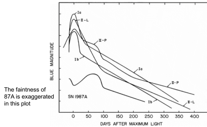
Fig. 1.5 A comparison of characteristic light curves. From “Introduction to Supernovae” (Wheeler 1990)
