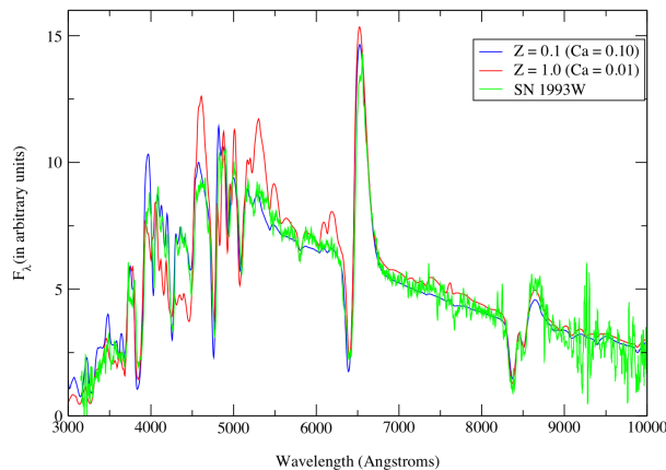
Modeling the spectrum of a Type II supernova in the Hubble flow (5400 km/s) by Baron et al. (2003). SN 1993W at 28 days. The spectrum suggests low metallicity.
