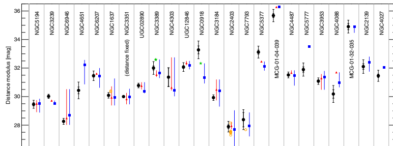
Figure 11. Comparison of the distance estimates of galaxies in our sample (solid black circles with 1\sigma uncertainties of the original fit and the modified fit with H_0/N_{\text{Dop}} = 1 ) to the data in NED; median values of either Type II supernovae only or all distance estimates are shown with solid red triangle or blue square, respectively, while the full range of measurements is shown with vertical colored lines. For a few galaxies, we highlight individual distance measurements with Cepheids (open orange circles) or with supernovae Ia (solid green stars). Distances of Type II supernovae are from Baron et al. (1996, 2007), Bartel (1988), Bose & Kumar (2014), Dessart & Hillier (2006); Dessart et al. (2008), Elmhamdi et al. (2003), Fraser et al. (2011), Hamuy et al. (2001), Hendry et al. (2006), Insearra et al. (2012a), Iwamoto et al. (1994), Jones et al. (2009), Leonard et al. (2002a, 2002b, 2003), Olivares E. et al. (2010), Poznanski et al. (2009), Richmond et al. (1996), Roy et al. (2011), Sahu et al. (2006), Schmidt et al. (1992, 1994a, 1994b), Sparks (1994), Takais et al. (2014), Takais & Vinkó (2006, 2012), Tomasella et al. (2013), Vinkó et al. (2006, 2012), Weiler et al. (1998), of Cepheids are from Freedman & Madore (1988), Freedman et al. (2001), Humphreys et al. (1986), Leonard et al. (2003), Madore & Freedman (1991), McAlary & Madore (1984), Metcalfe & Shanks (1991), Pietrzyński et al. (2010), Saha et al. (2006), and of Type Ia supernovae from: Maguire et al. (2012), Parodi et al. (2000).
