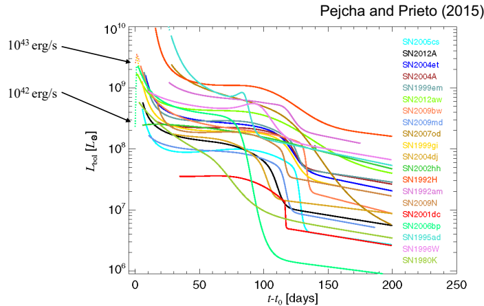
Figure 14. Bolometric luminosity as a function of time for supernovae with \sigma_\mu < 0.2 mag. The bolometric luminosity was calculated from the UBVRIZHK bands combined with Swift bands uvw2 , uvm2 , uvw1 , and u . For each supernova, we show L_{bol} between the first and last observation. Dotted segments of L_{bol} mark the temperatures not constrained by Swift data ( \tau < 0.095 ).
