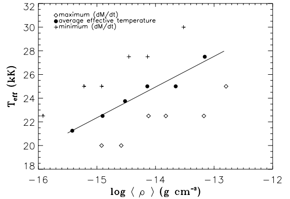
Fig. 3. Characteristic density \log \langle \rho \rangle and T_{\text{eff}} of the bi-stability jump around T_{\text{eff}} = 25 000 K. An explanation for the different symbols is given in the legend. The solid line represents the best linear fit through the average jump parameters \log \langle \rho \rangle and T_{\text{eff}}
