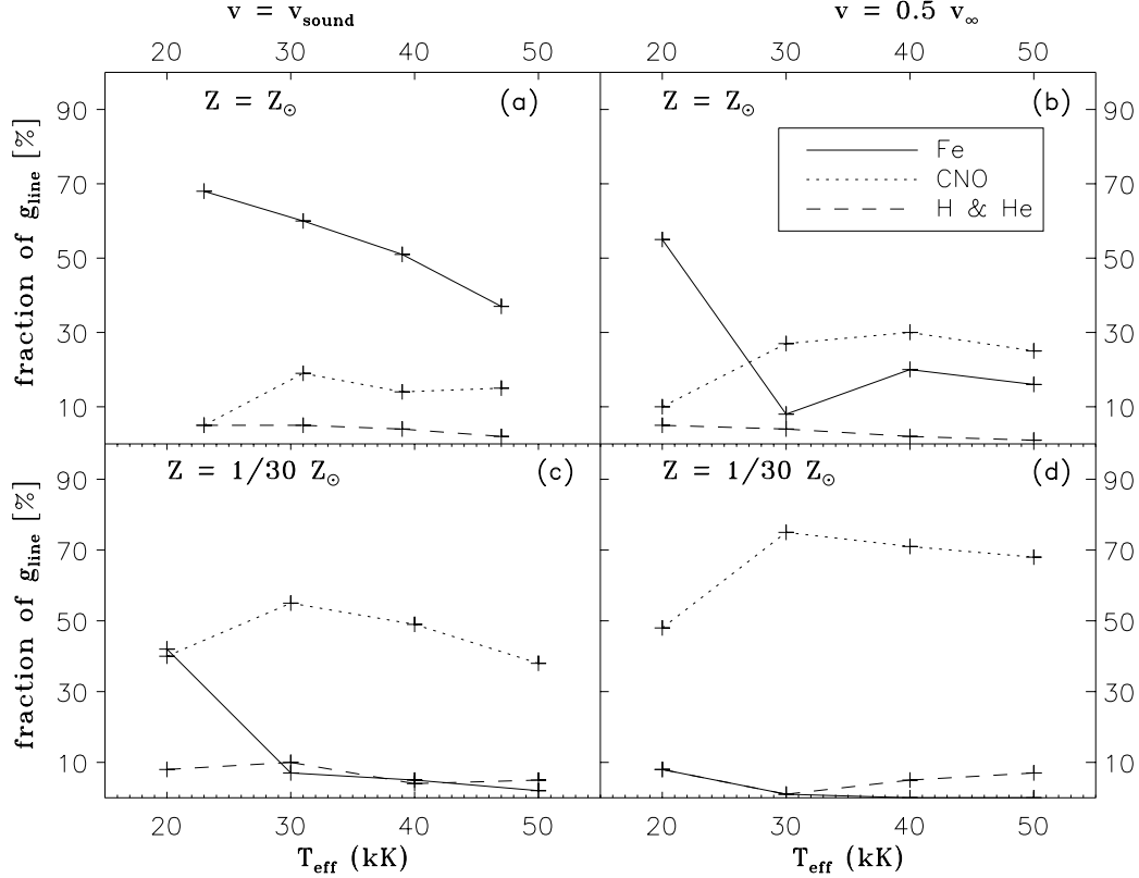
Fig. 4. The relative contribution to the line acceleration for models with (v_{\infty}/v_{\text{esc}}) = 2.0 , \log L_*/L_{\odot} = 5.5 and M_* = 40 M_{\odot} . The solid lines show the contribution of Fe lines. The dotted line is the contribution by C, N and O. The dashed line shows the contribution by H and He lines. a) and b) give the contribution for solar Z at resp. v = v_{\text{sound}} and at v = 0.5v_{\infty} . c) and d) give the contribution for (Z/Z_{\odot}) = 1/30 at resp. v = v_{\text{sound}} and at v = 0.5v_{\infty} .
